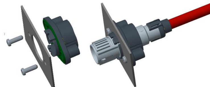
Mounting Flange
